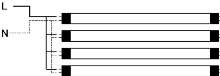
Fig. C: Ballast Bypass - Multiple Tubes
