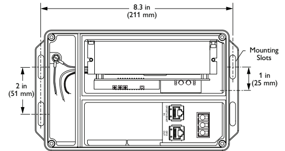
Mounting Dimensions
