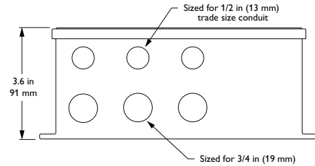
Overall Dimensions
