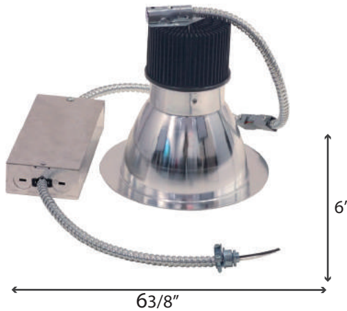
6" LED Commercial Recessed Downlight Retrofits
