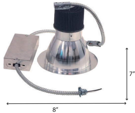
8" LED Commercial Recessed Downlight Retrofits
